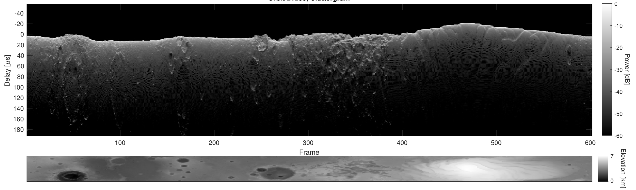
Orbit 21288, Cluttergram
