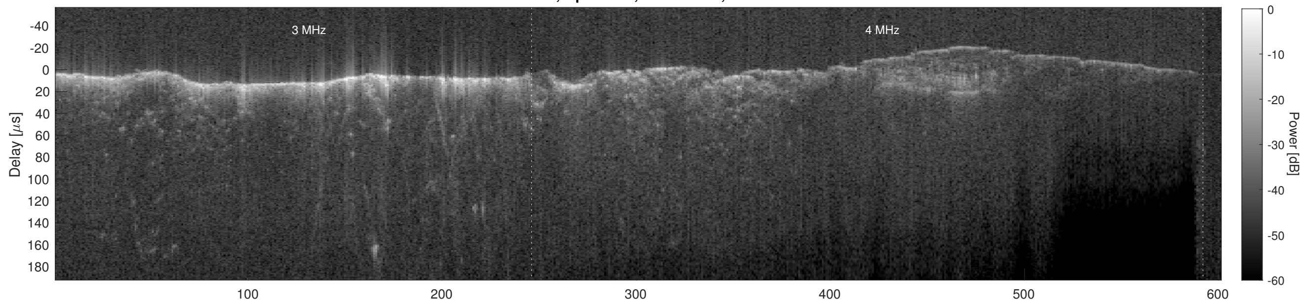
Orbit 21288, Cluttergram
