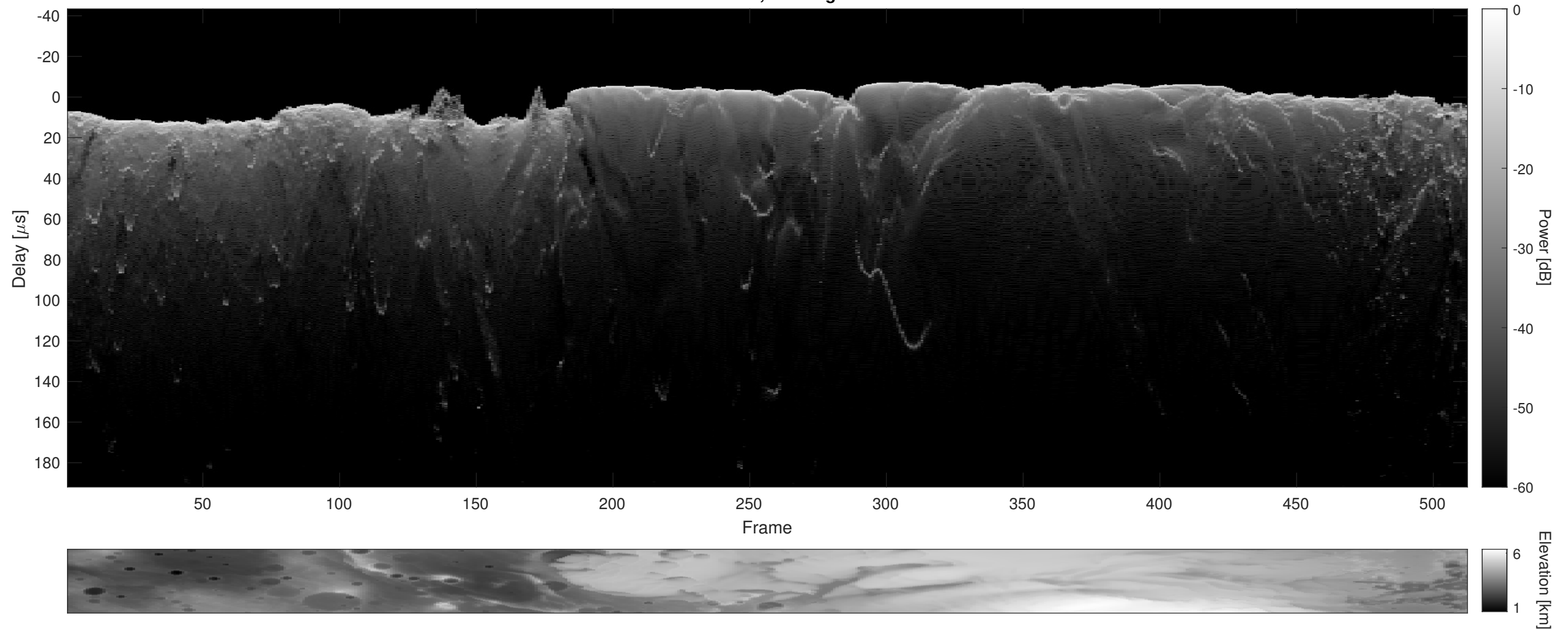
Orbit 21293, Cluttergram
