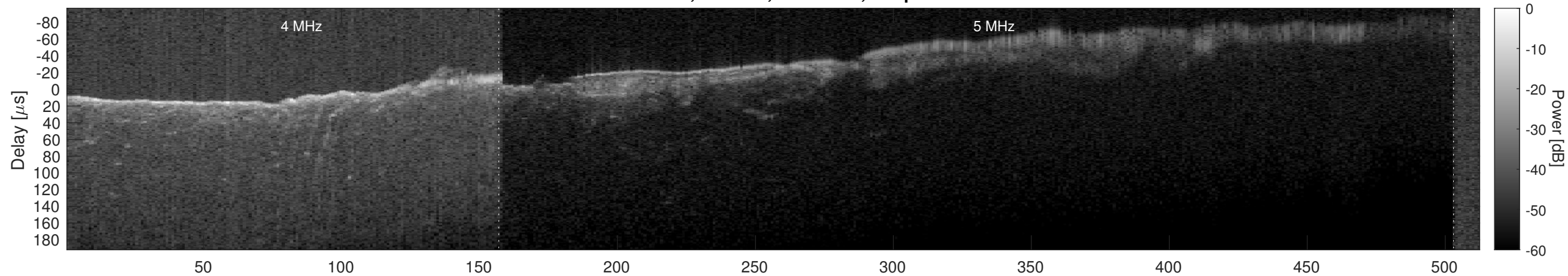
Orbit 21293, Window, Channel 1, Optimized
