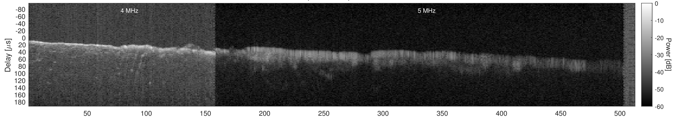
Orbit 21293, Window, Channel 1, Chapman
