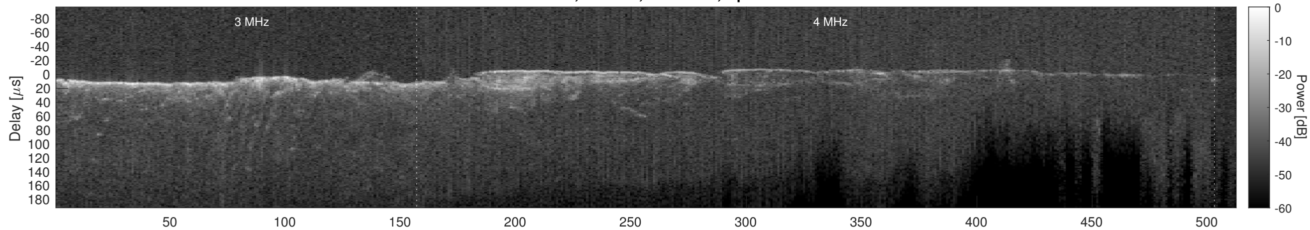
Orbit 21293, Cluttergram
