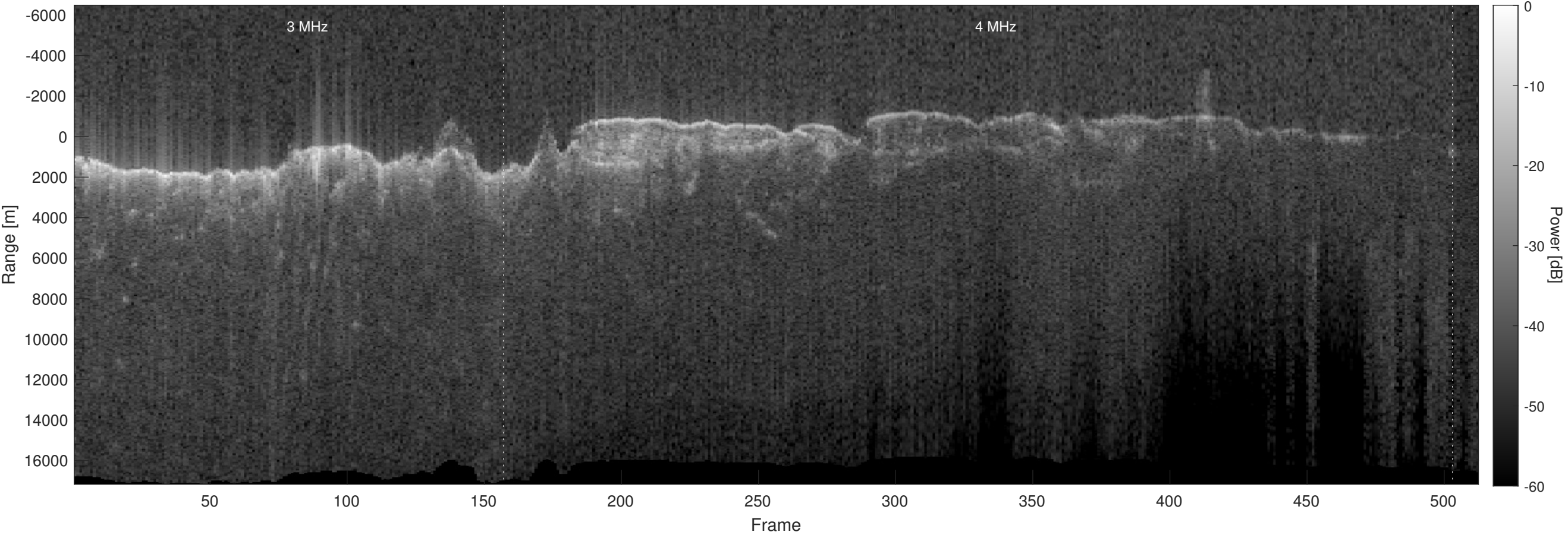
Orbit 21293, Optimized, No Window, Depth-Corrected, Channel 2
