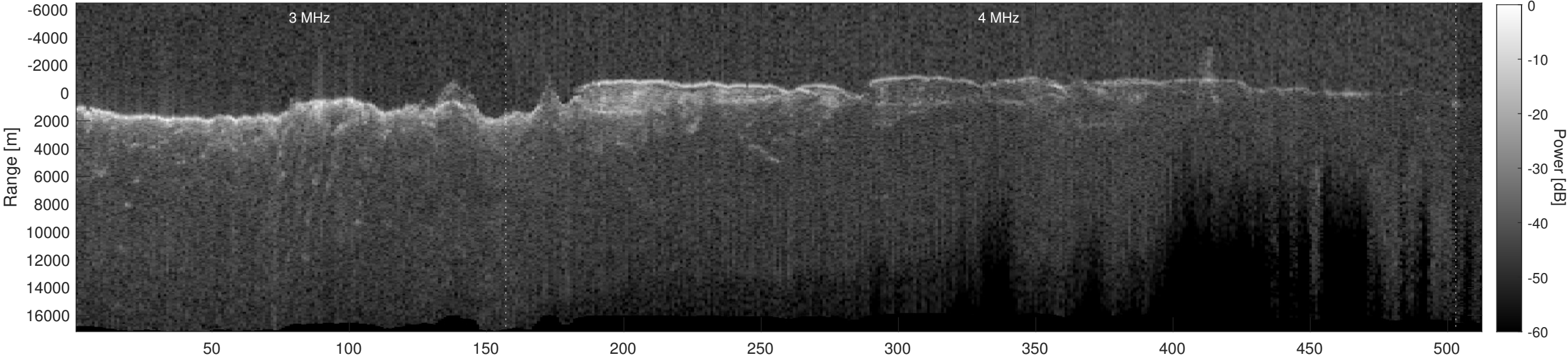
Orbit 21293, Depth-Corrected Cluttergram
