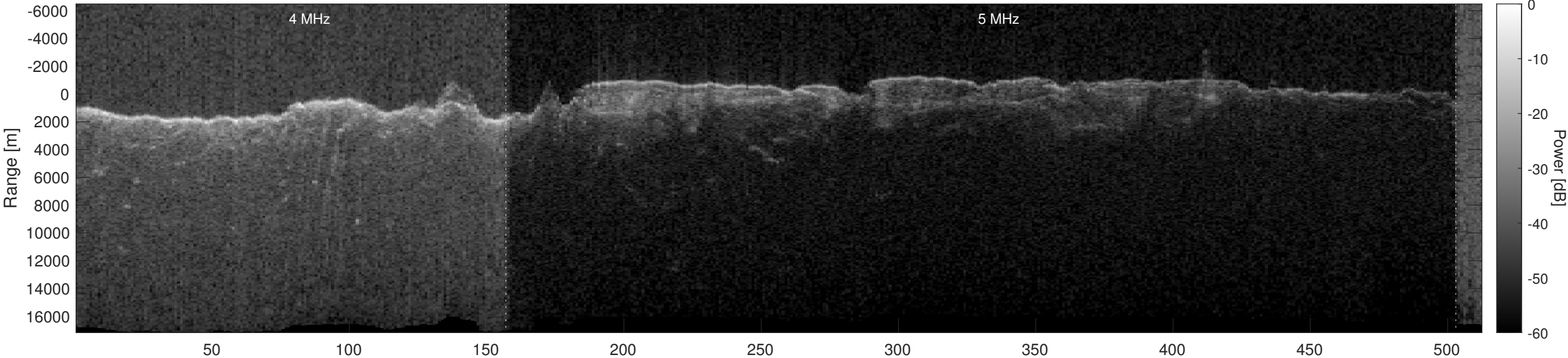
Orbit 21293, Optimized, Window, Depth-Corrected, Channel 2
