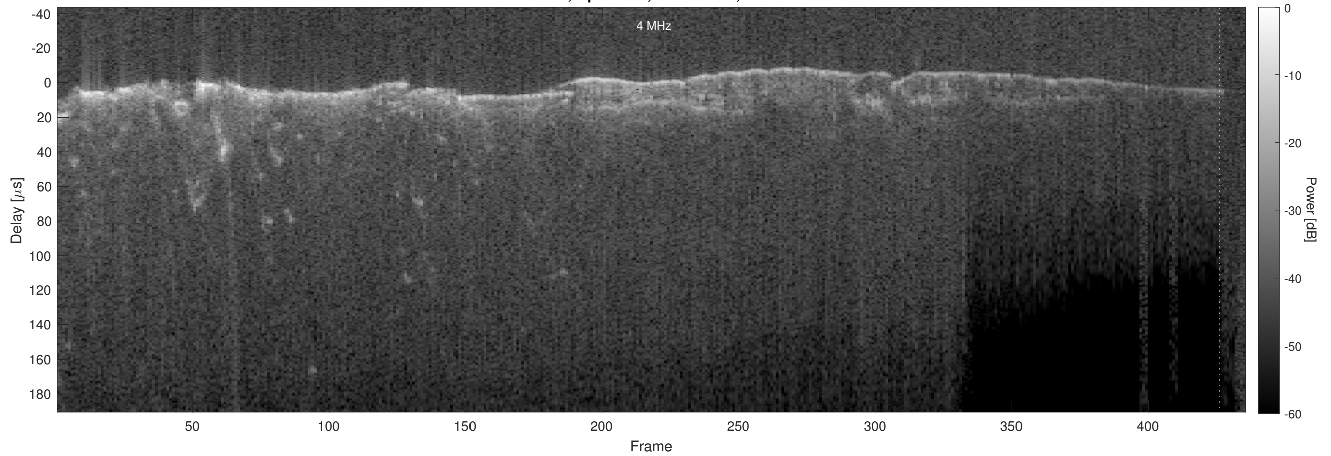
Orbit 21304, Optimized, No Window, Channel 2
