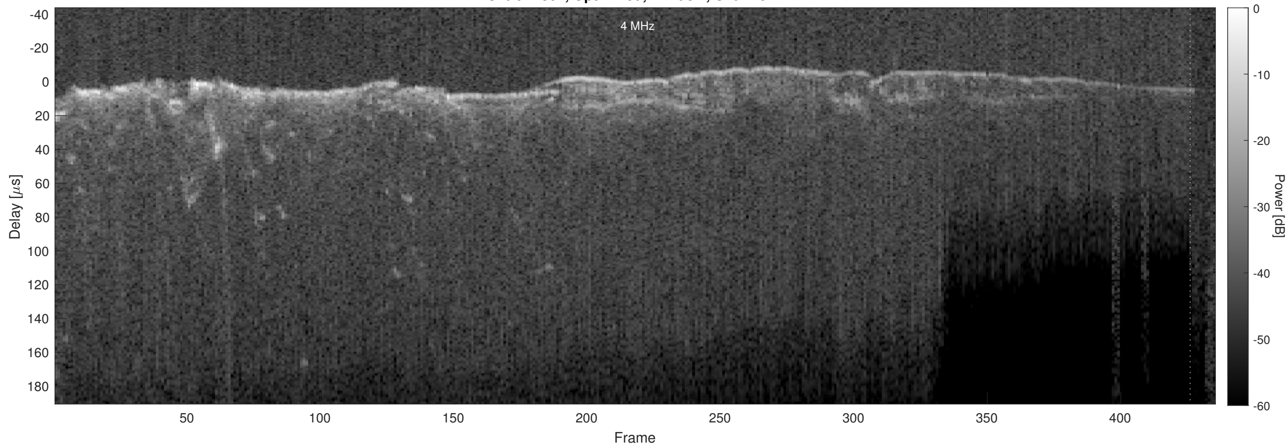
Orbit 21304, Optimized, Window, Channel 2
