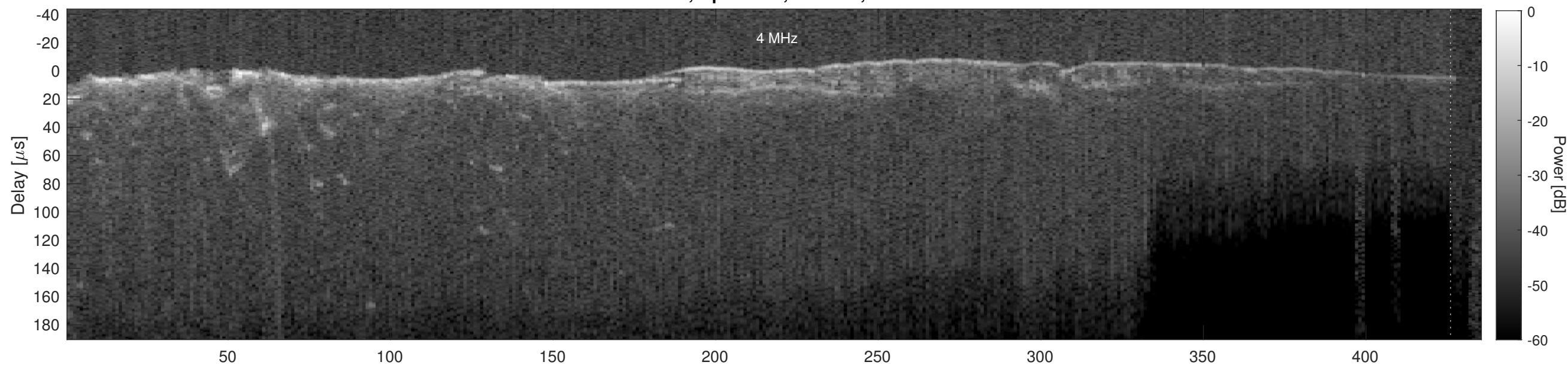
Orbit 21304, Cluttergram
