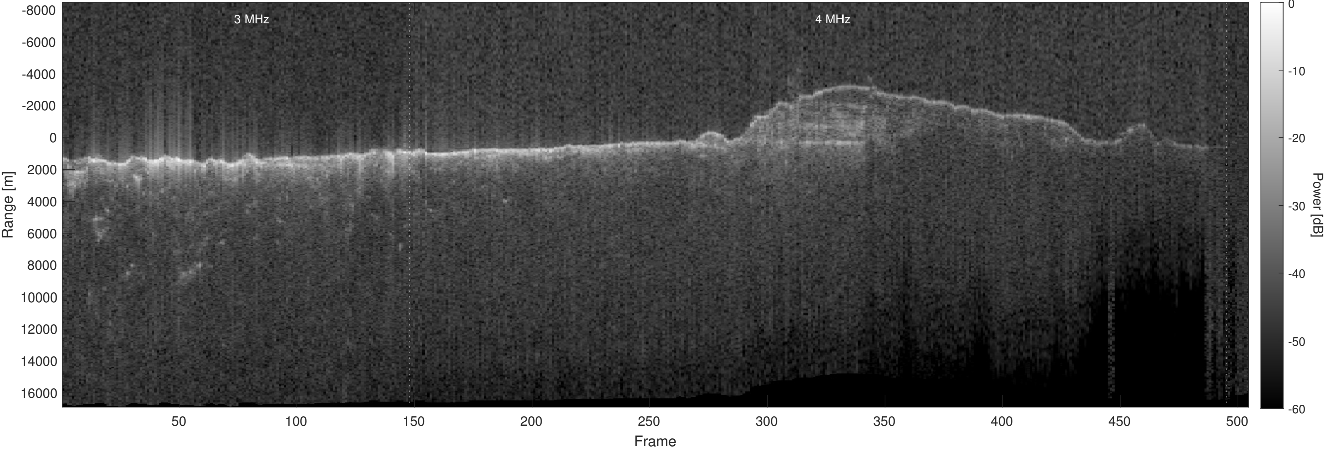
Orbit 21316, Optimized, No Window, Depth-Corrected, Channel 2
