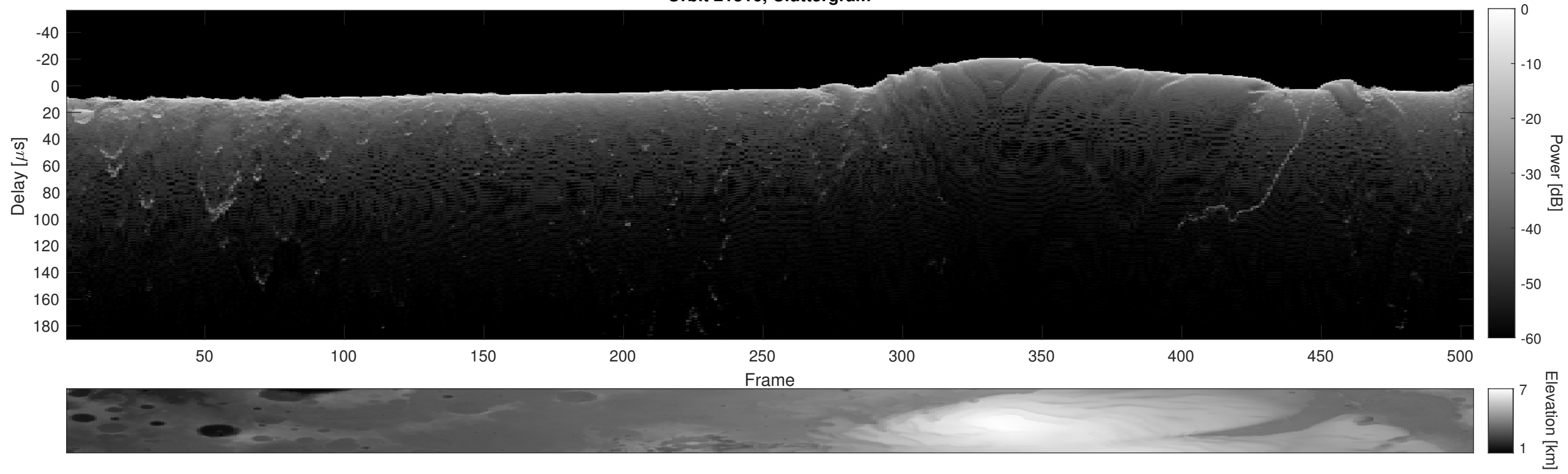
Orbit 21316, Cluttergram
