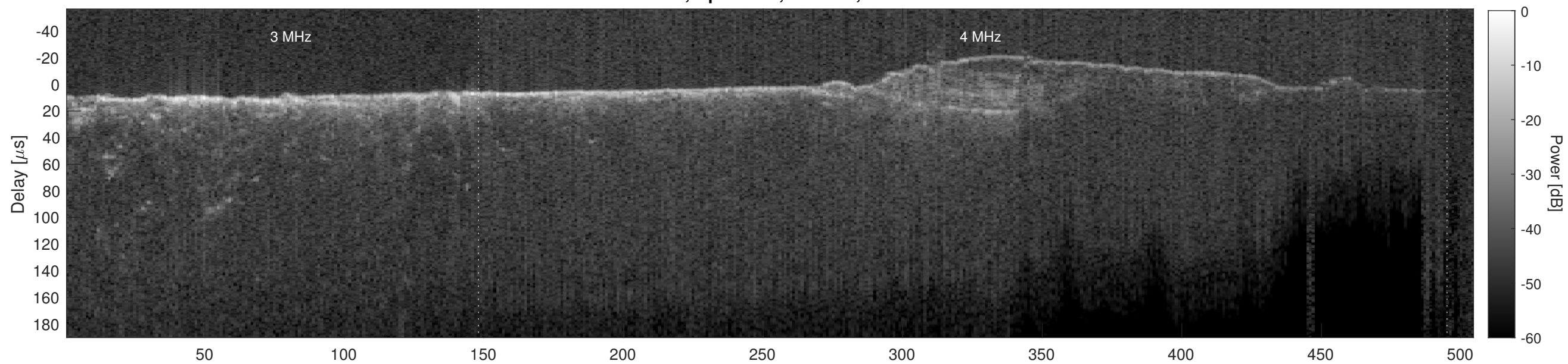
Orbit 21316, Cluttergram
