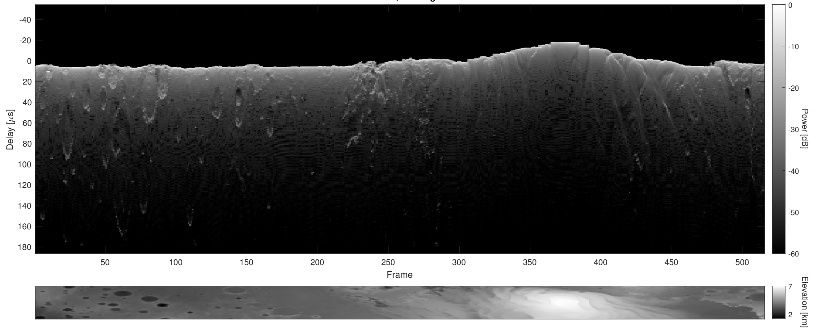
Orbit 21320, Cluttergram
