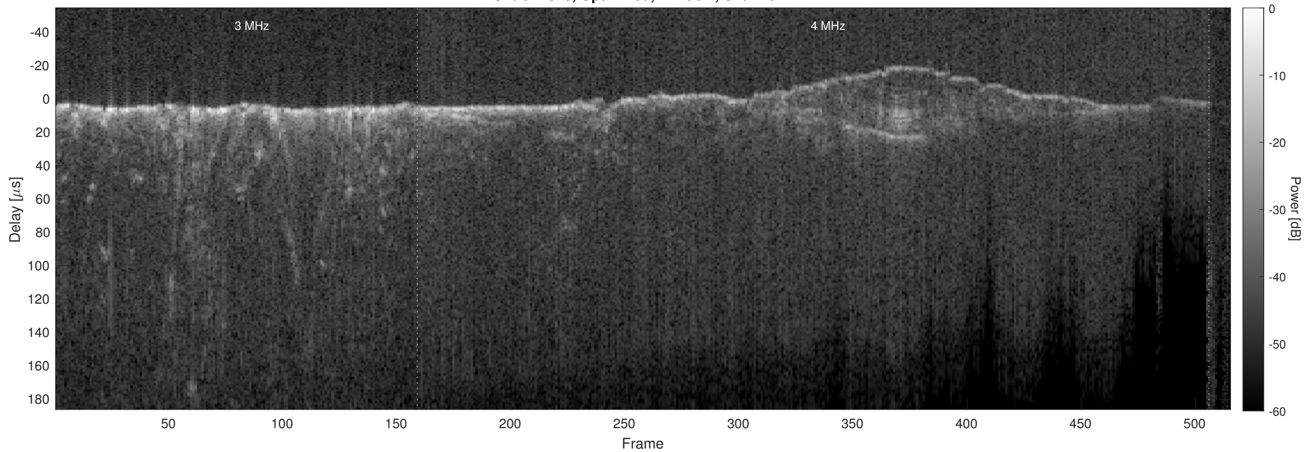
Orbit 21320, Optimized, Window, Channel 2
