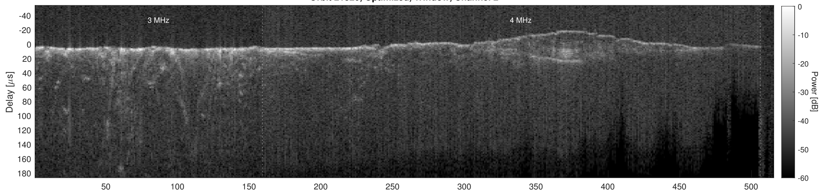
Orbit 21320, Cluttergram
