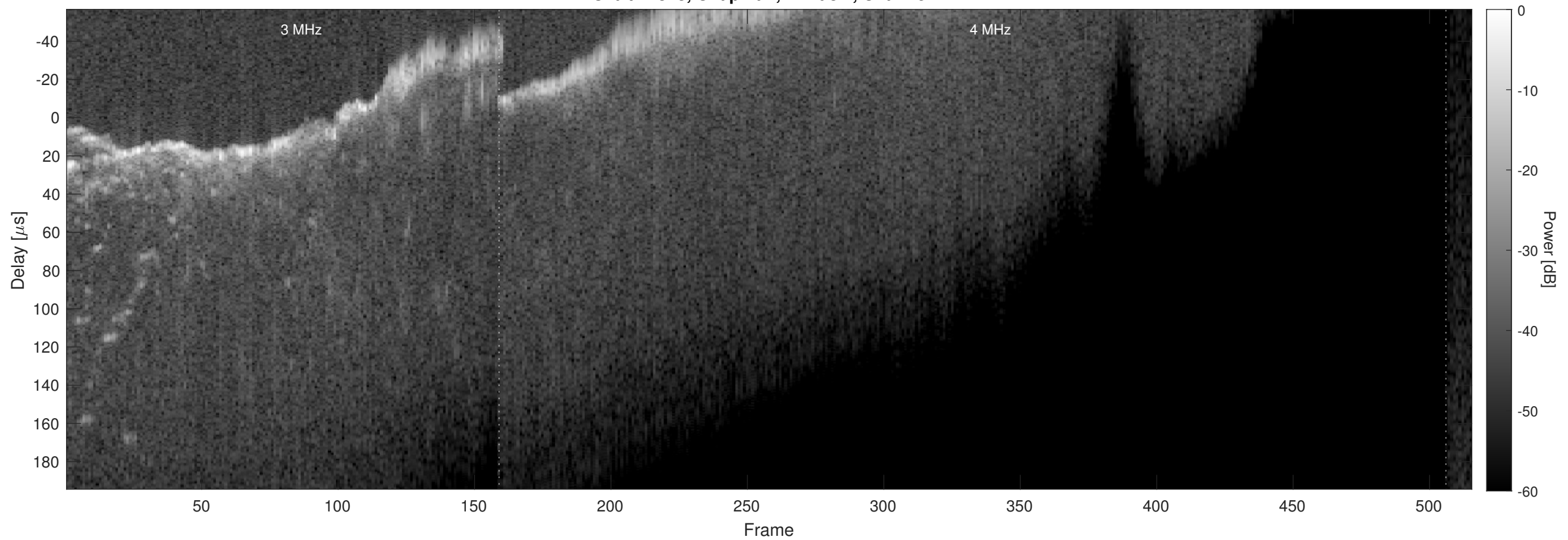
Orbit 21323, Chapman, Window, Channel 2
