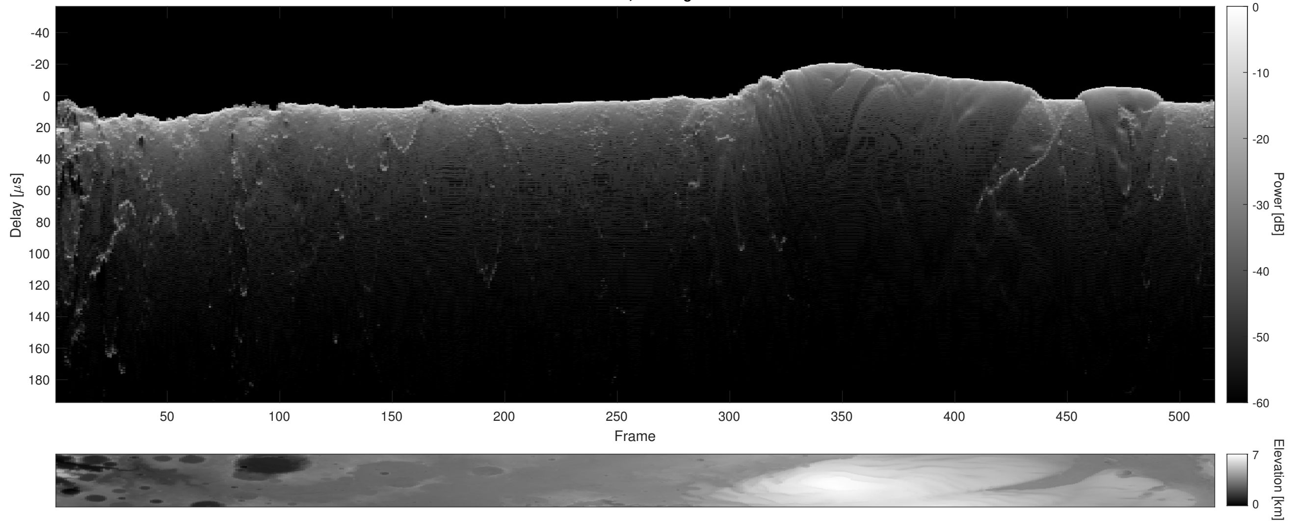
Orbit 21323, Cluttergram
