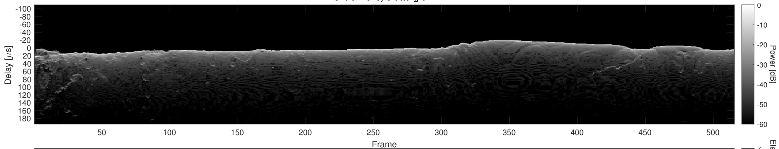
Orbit 21323, Cluttergram
