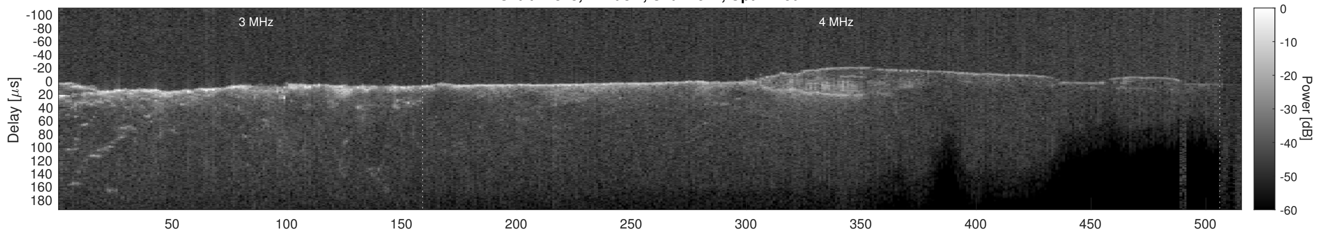
Orbit 21323, Cluttergram
