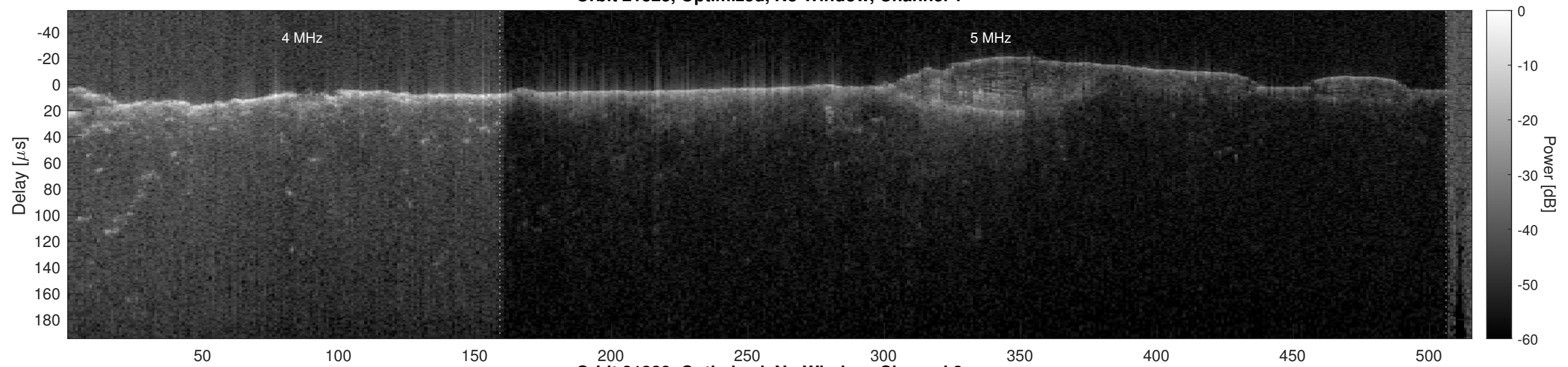
Orbit 21323, Optimized, No Window, Channel 2
