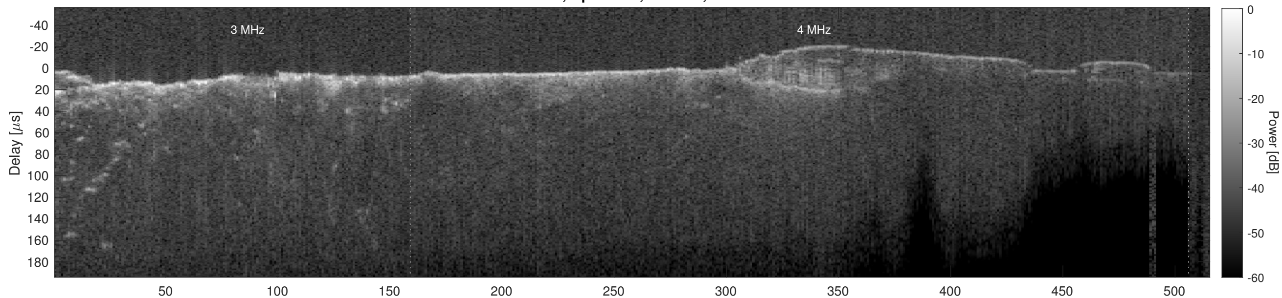
Orbit 21323, Cluttergram
