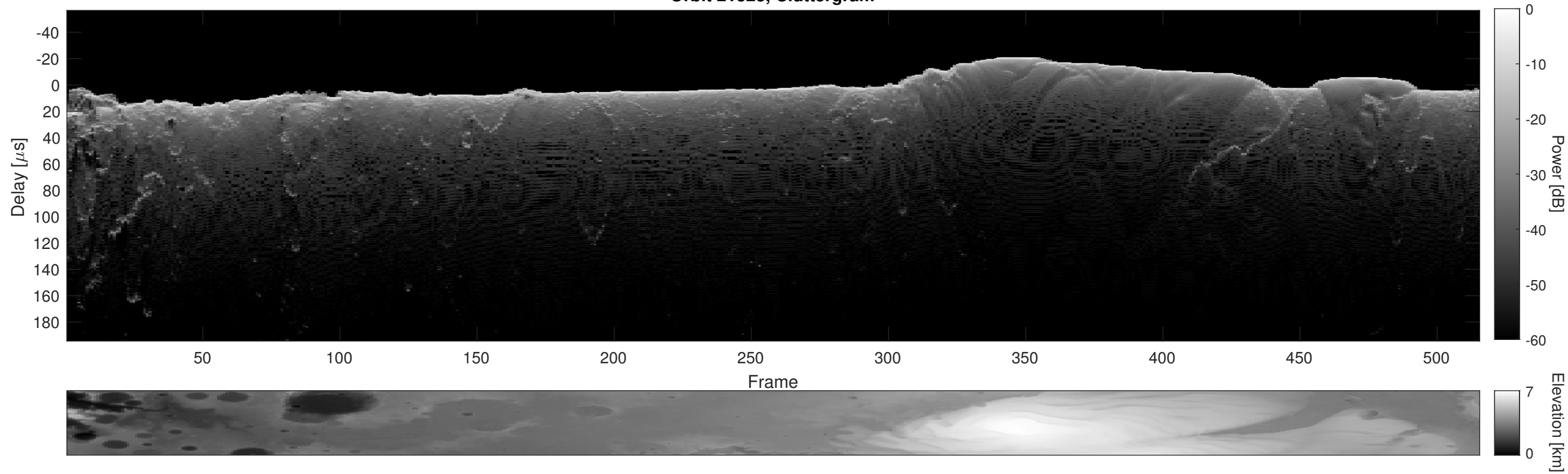
Orbit 21323, Cluttergram
