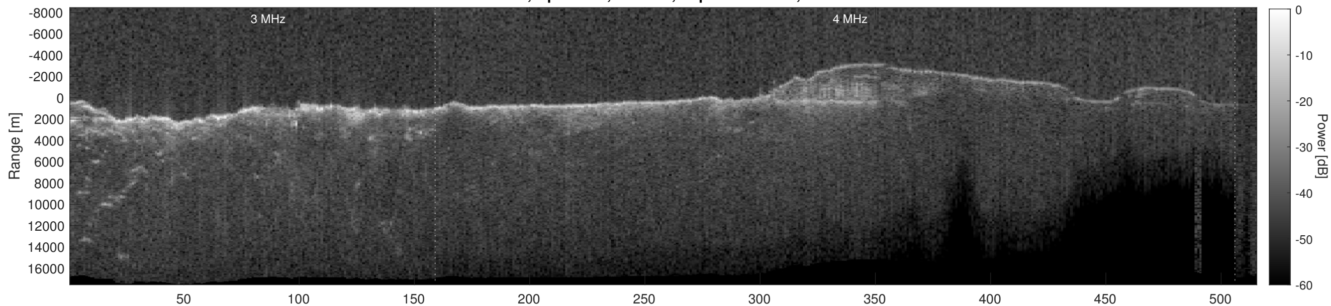
Orbit 21323, Depth-Corrected Cluttergram
