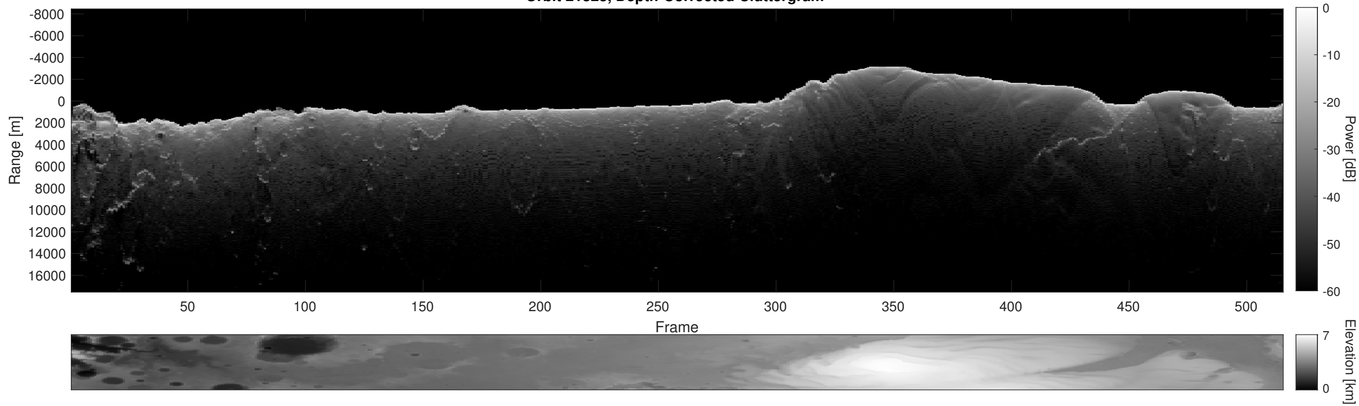
Orbit 21323, Depth-Corrected Cluttergram
