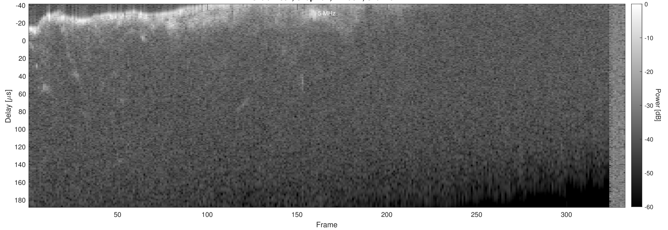
Orbit 21332, Chapman, Window, Channel 2
