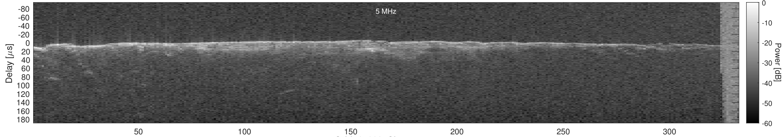
Orbit 21332, Cluttergram
