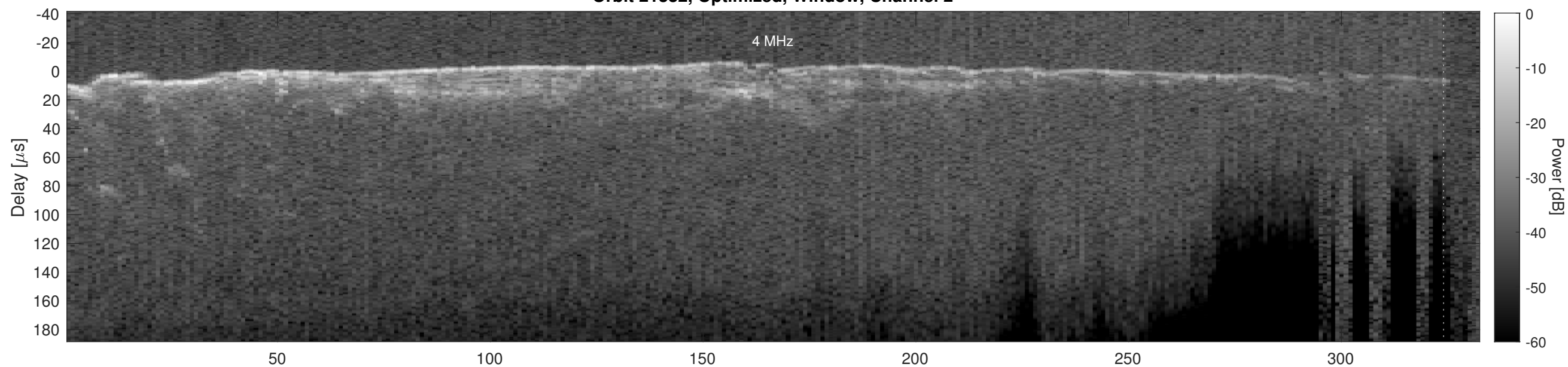
Orbit 21332, Cluttergram
