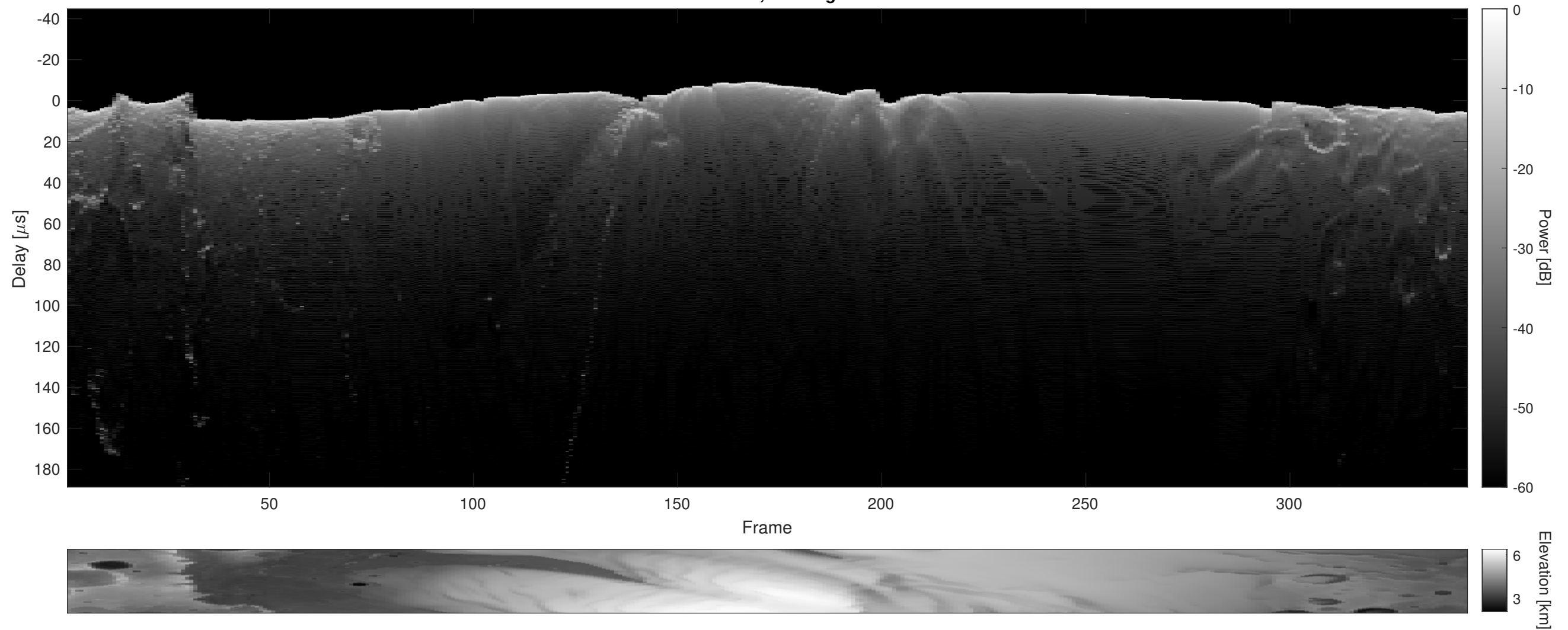
Orbit 21336, Cluttergram
