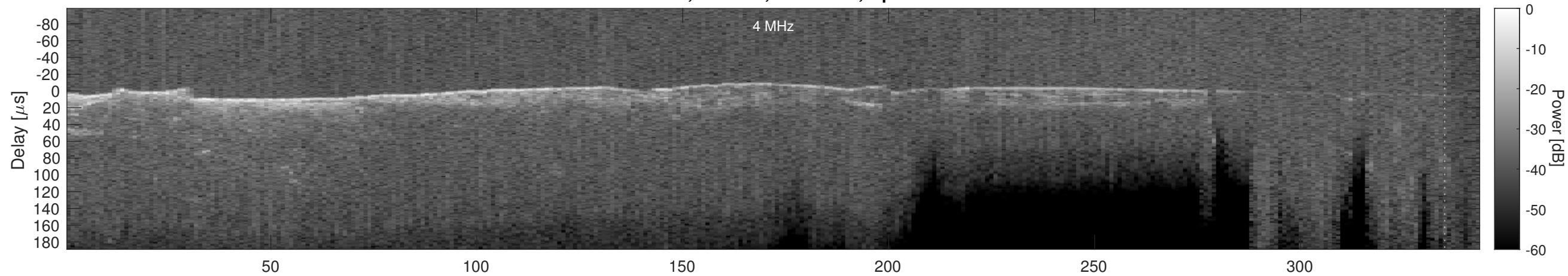
Orbit 21336, Cluttergram
