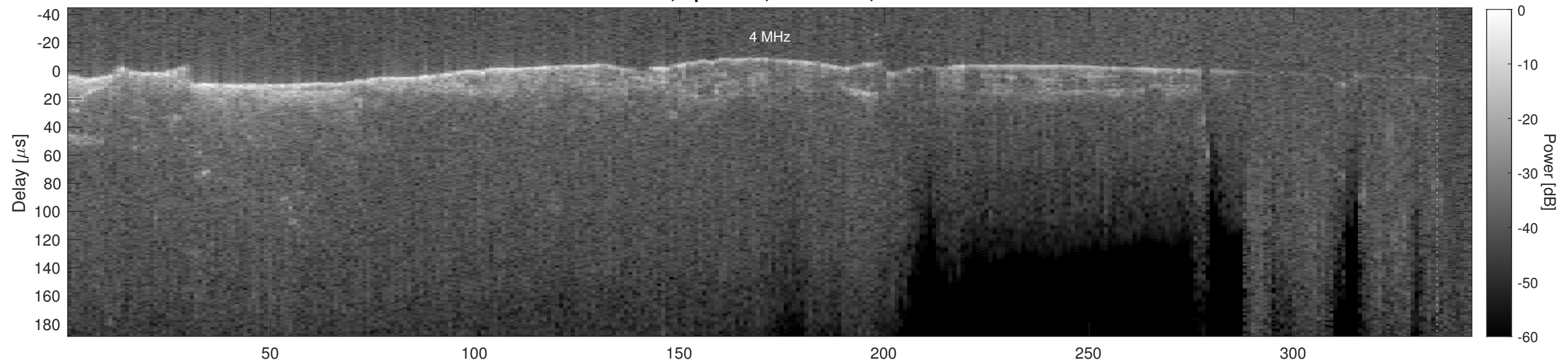
Orbit 21336, Cluttergram
