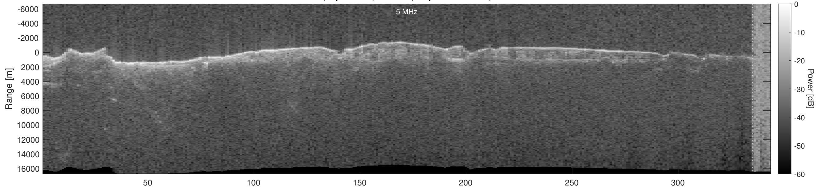
Orbit 21336, Optimized, Window, Depth-Corrected, Channel 2
