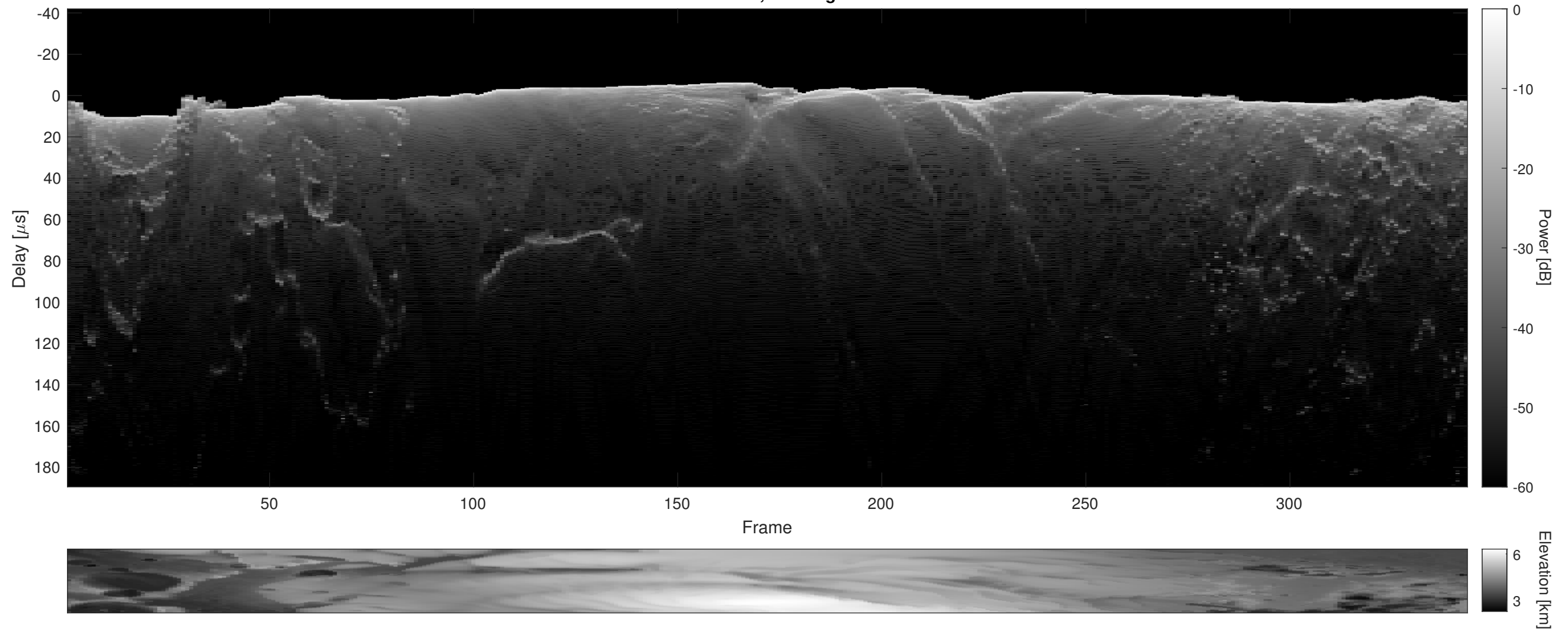
Orbit 21339, Cluttergram
