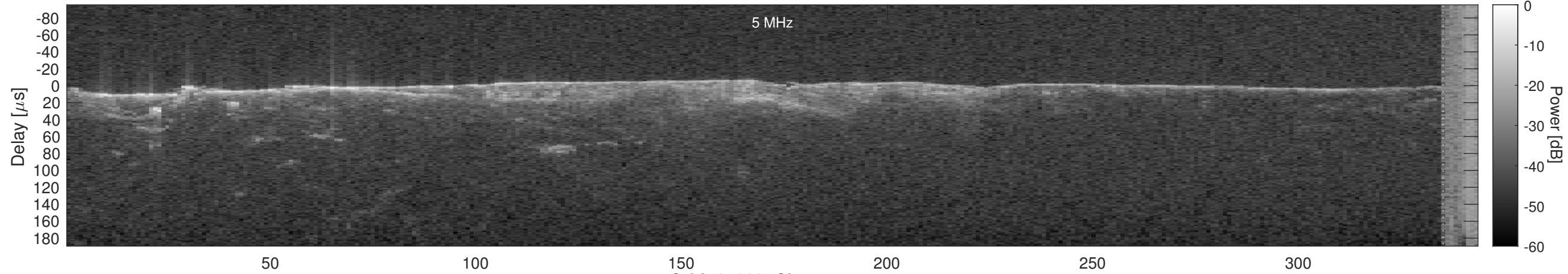
Orbit 21339, Cluttergram
