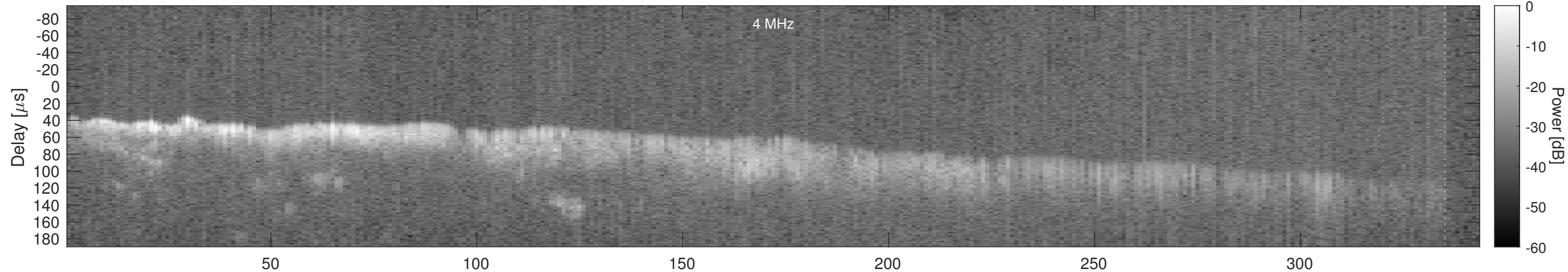
Orbit 21339, Window, Channel 2, Chapman
