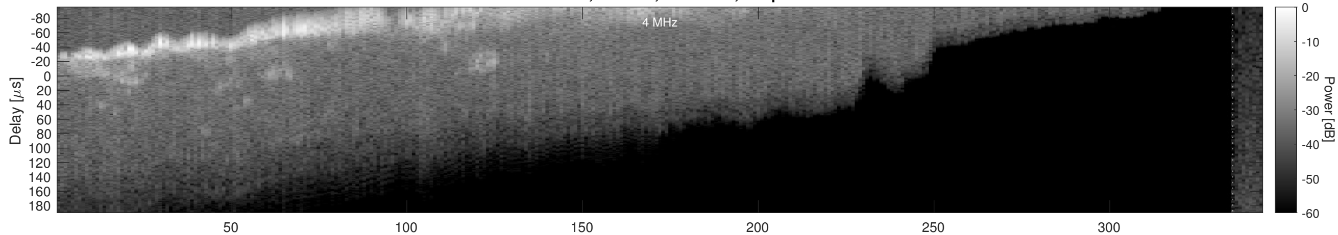
Orbit 21339, Window, Channel 2, Optimized
