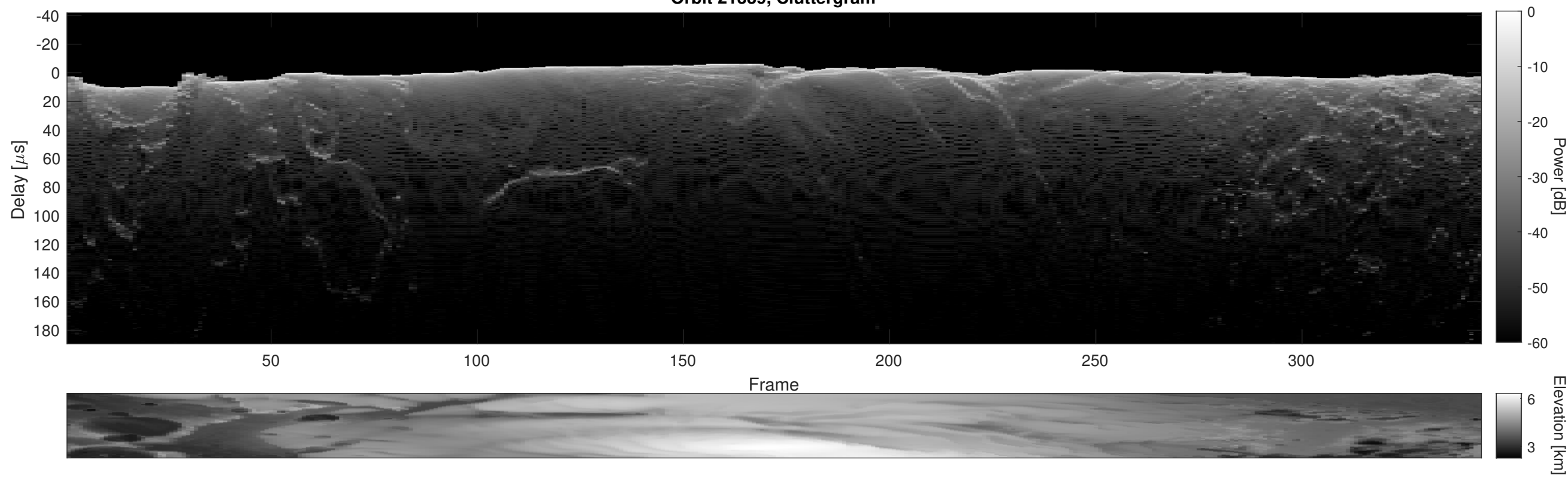
Orbit 21339, Cluttergram
