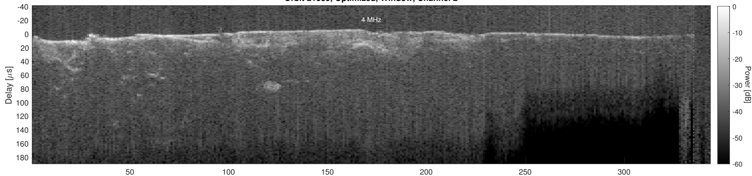
Orbit 21339, Cluttergram
