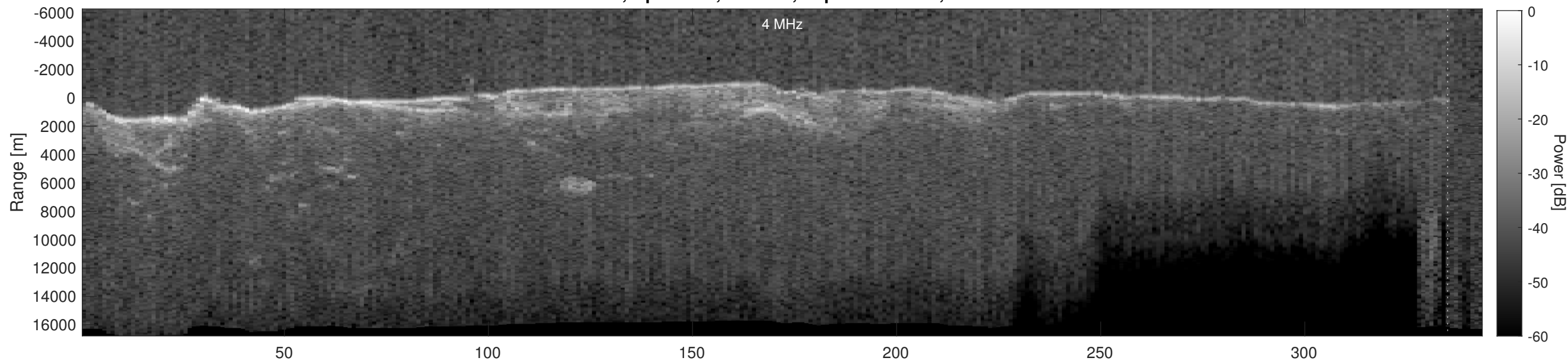
Orbit 21339, Depth-Corrected Cluttergram
