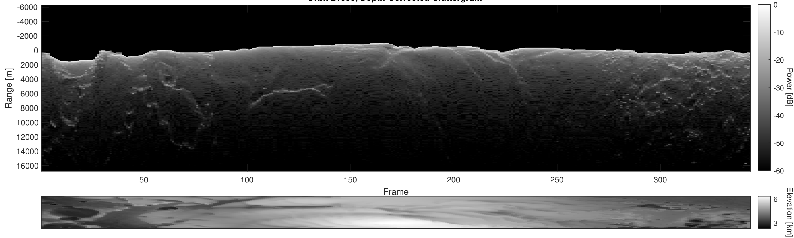
Orbit 21339, Depth-Corrected Cluttergram
