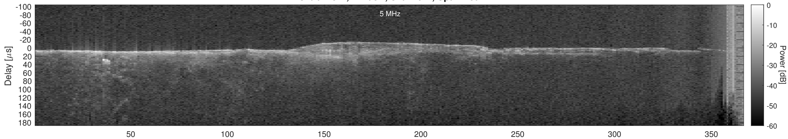
Orbit 21344, Cluttergram
