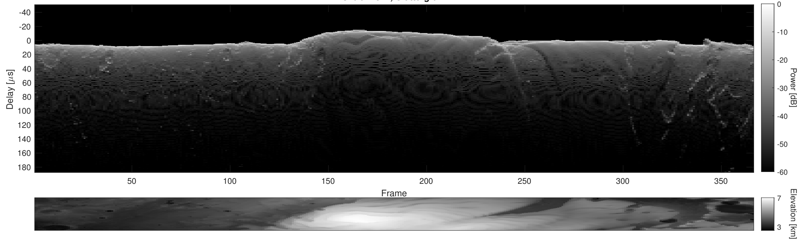
Orbit 21344, Cluttergram
