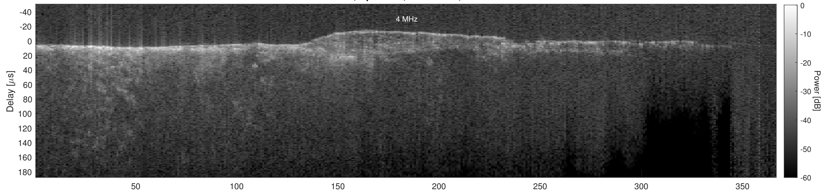
Orbit 21344, Cluttergram
