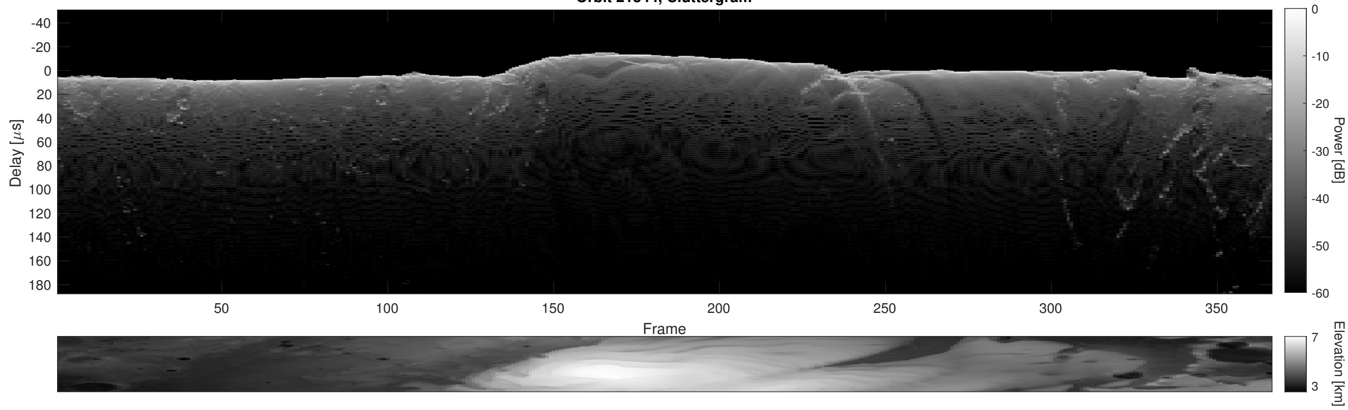
Orbit 21344, Cluttergram
