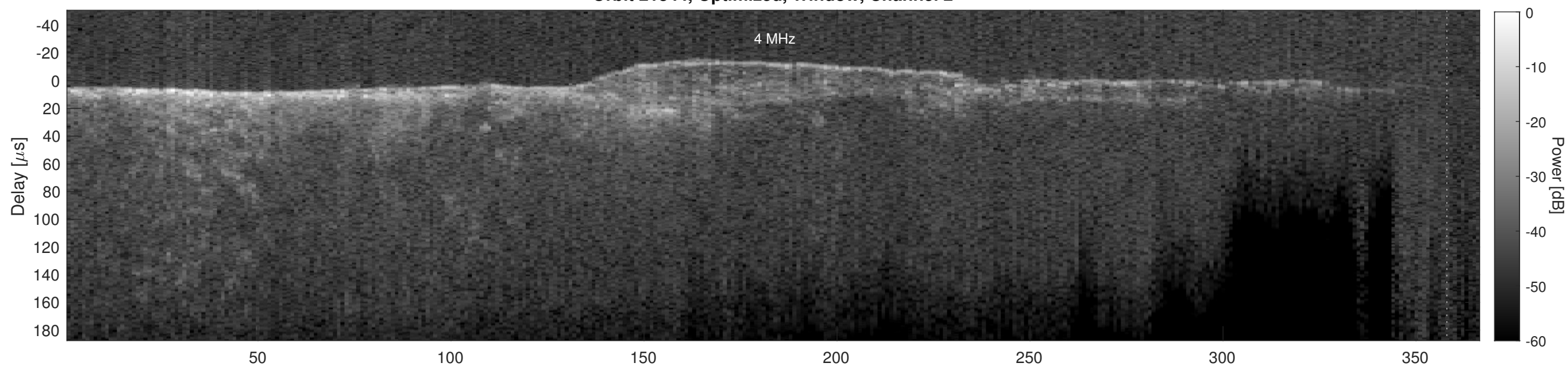
Orbit 21344, Cluttergram
