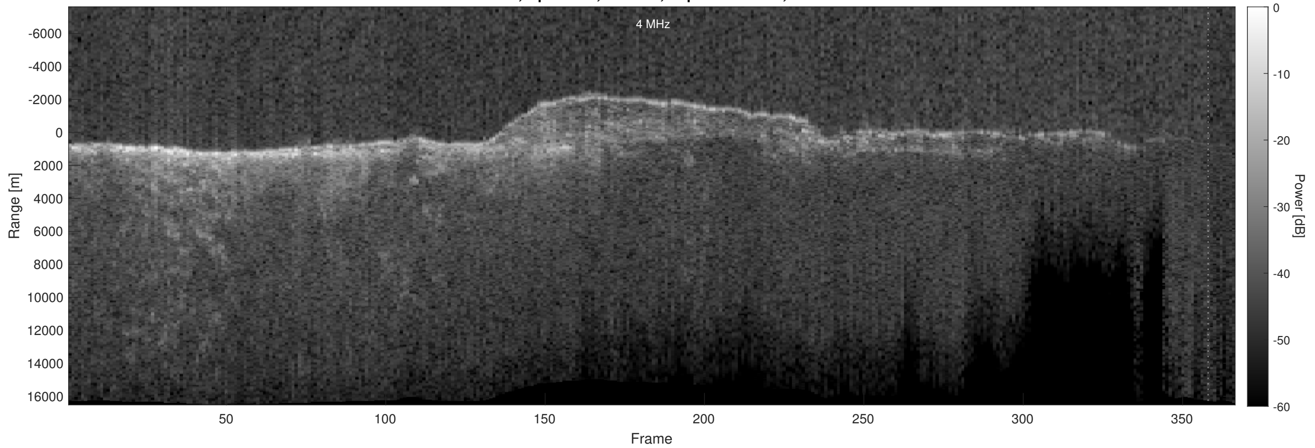
Orbit 21344, Optimized, Window, Depth-Corrected, Channel 2
