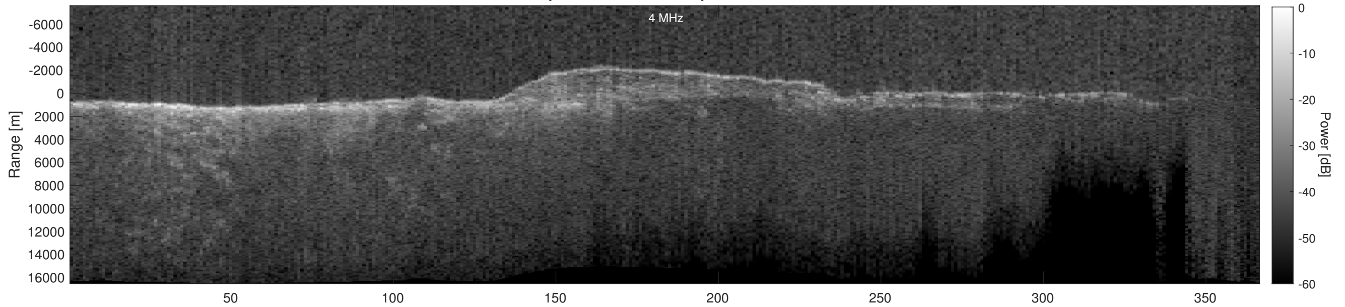
Orbit 21344, Depth-Corrected Cluttergram
