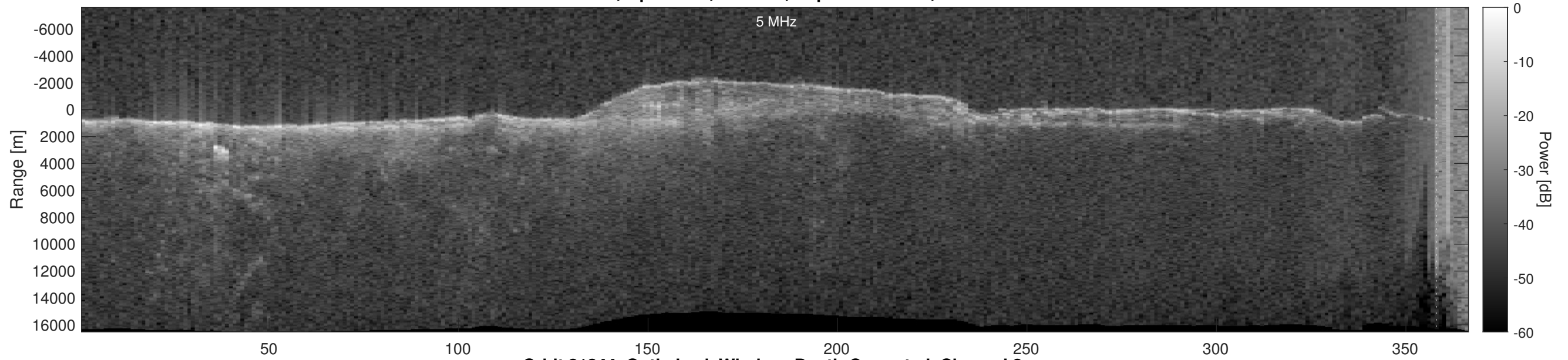
Orbit 21344, Optimized, Window, Depth-Corrected, Channel 2
