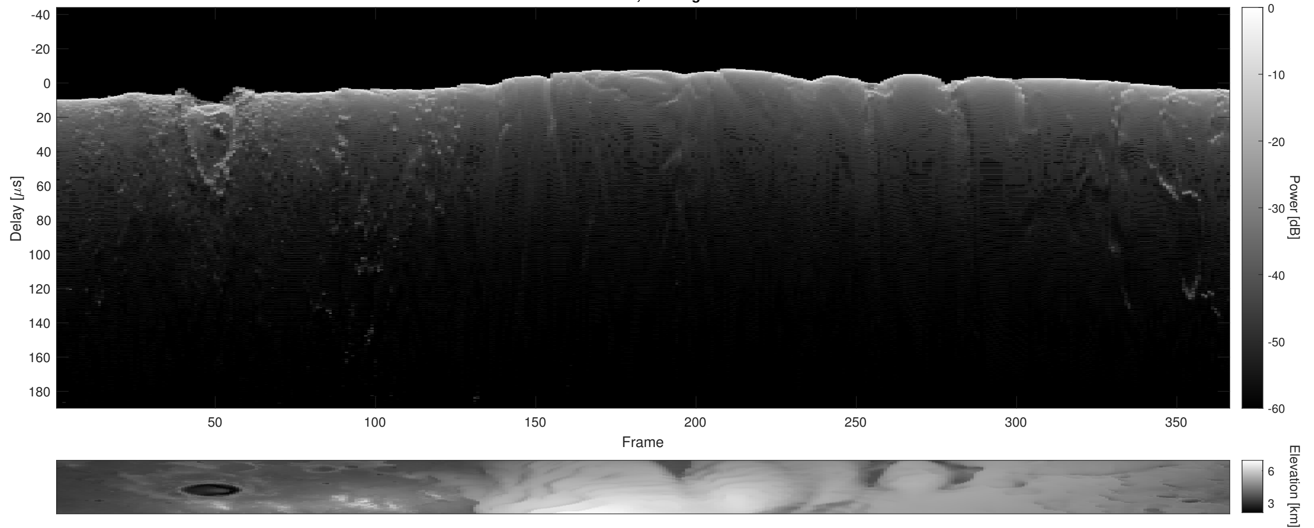
Orbit 21347, Cluttergram
