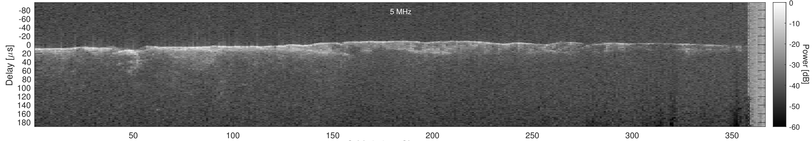
Orbit 21347, Cluttergram
