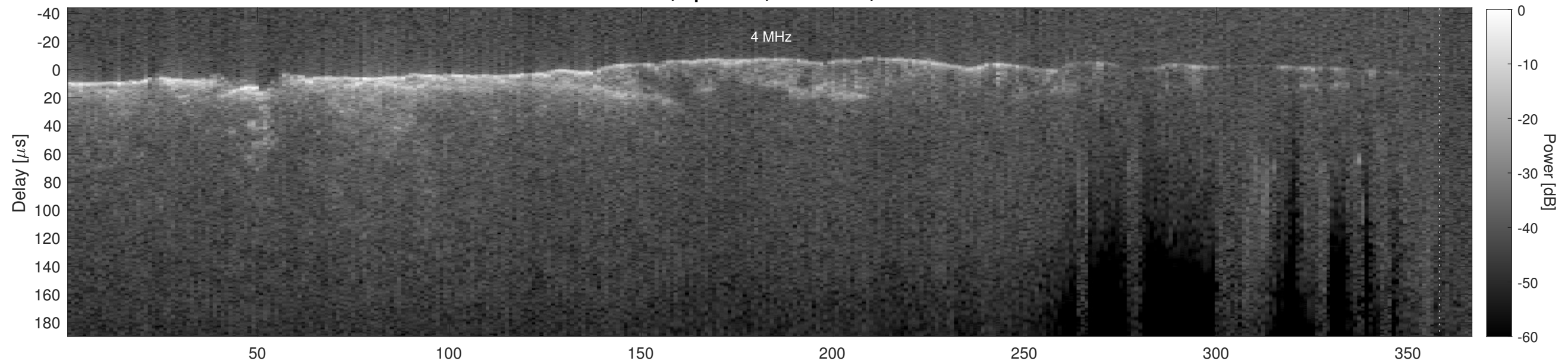
Orbit 21347, Cluttergram
