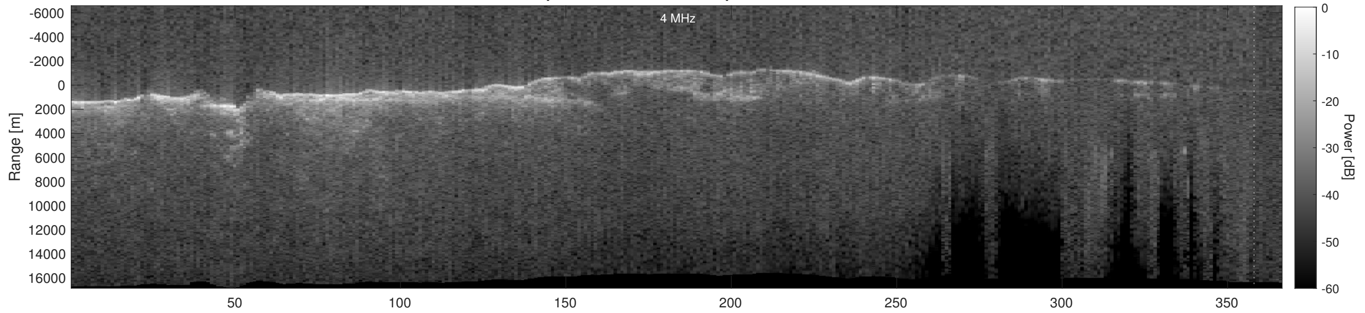
Orbit 21347, Depth-Corrected Cluttergram
