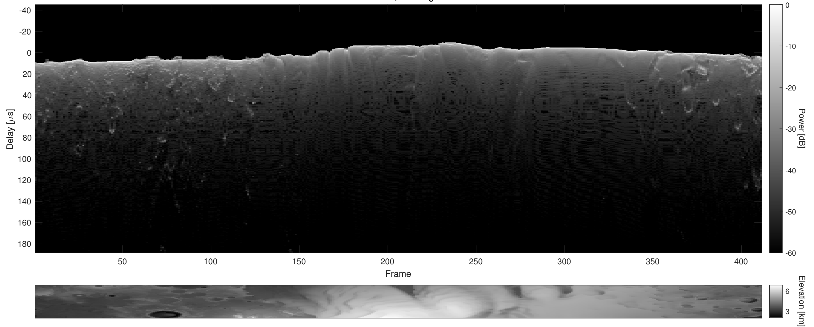
Orbit 21361, Cluttergram
