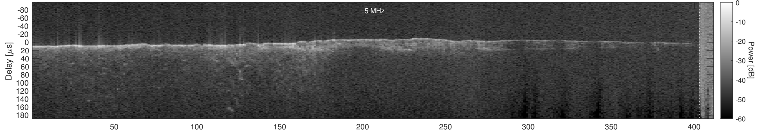
Orbit 21361, Cluttergram
