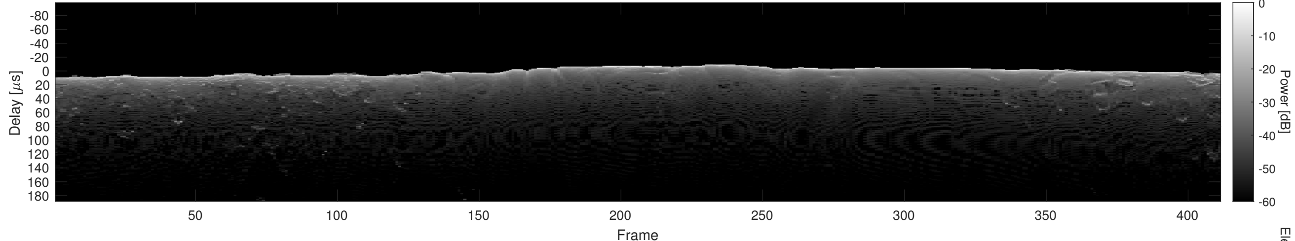
Orbit 21361, Cluttergram
