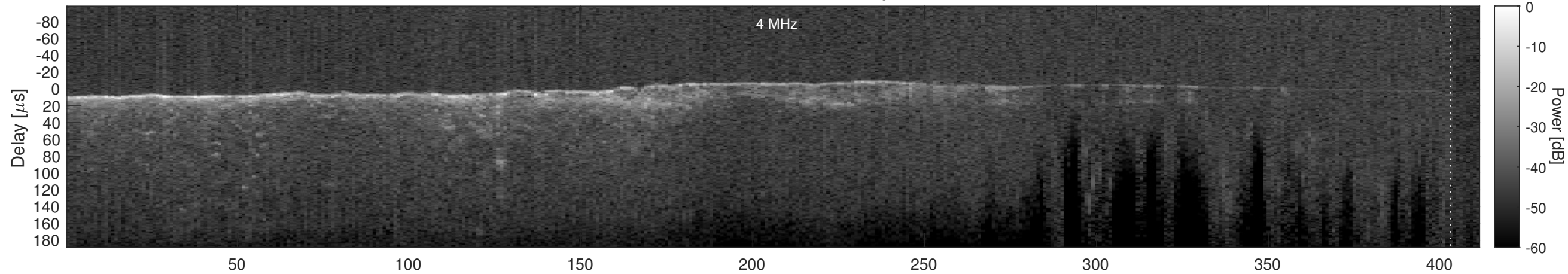
Orbit 21361, Cluttergram
