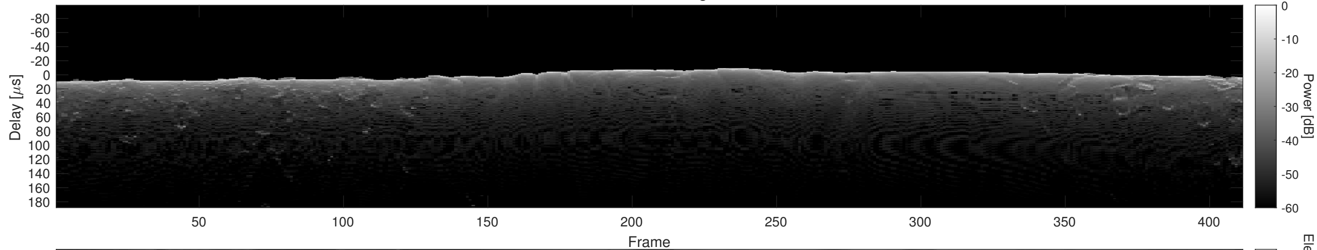
Orbit 21361, Cluttergram
