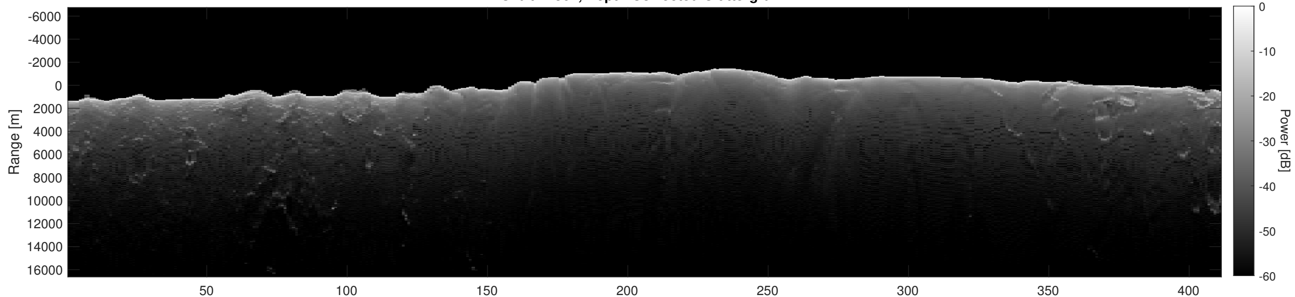
Orbit 21361, Depth-Corrected Cluttergram
