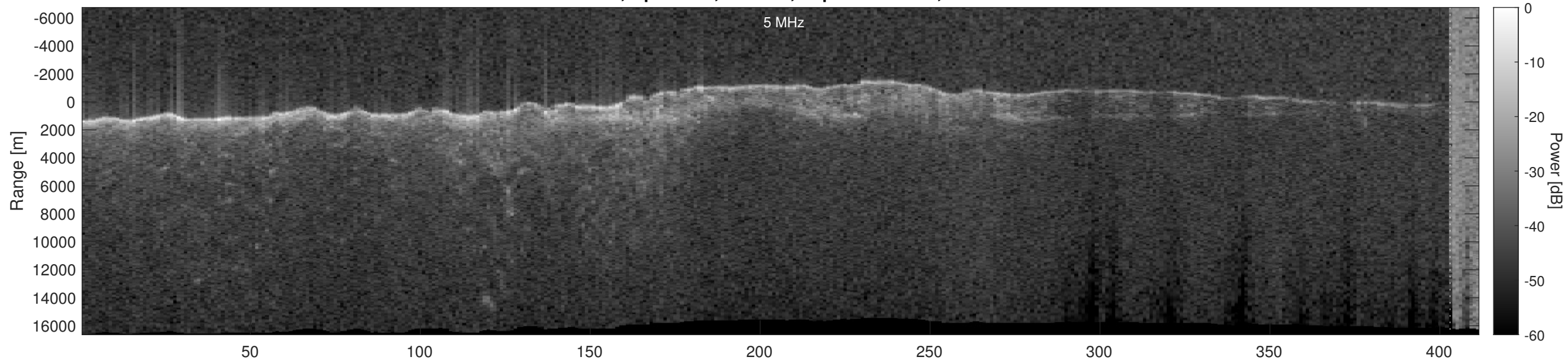
Orbit 21361, Optimized, Window, Depth-Corrected, Channel 2
