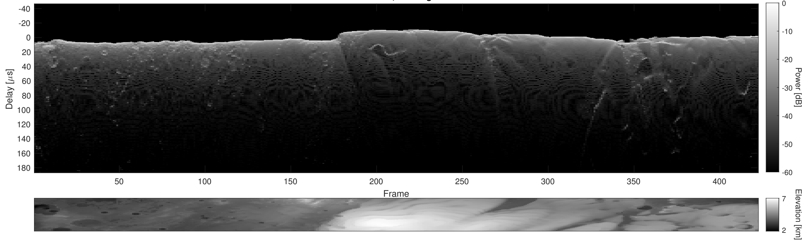
Orbit 21365, Cluttergram
