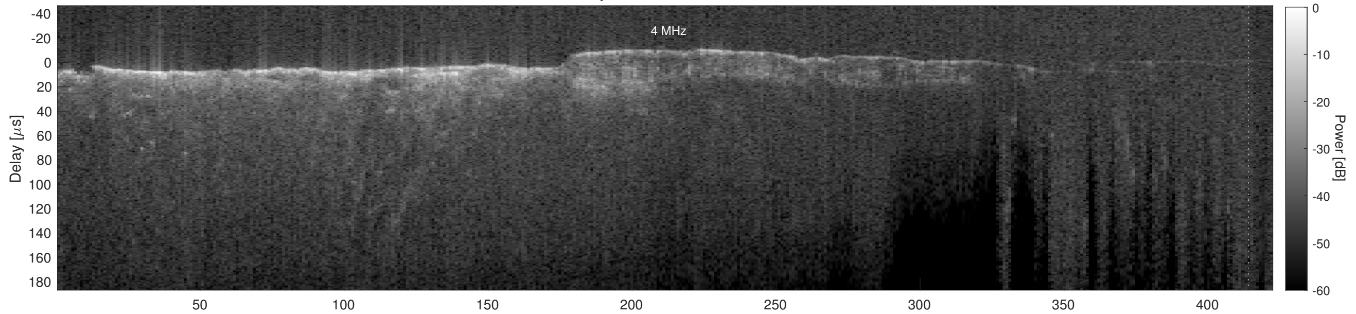
Orbit 21365, Cluttergram
