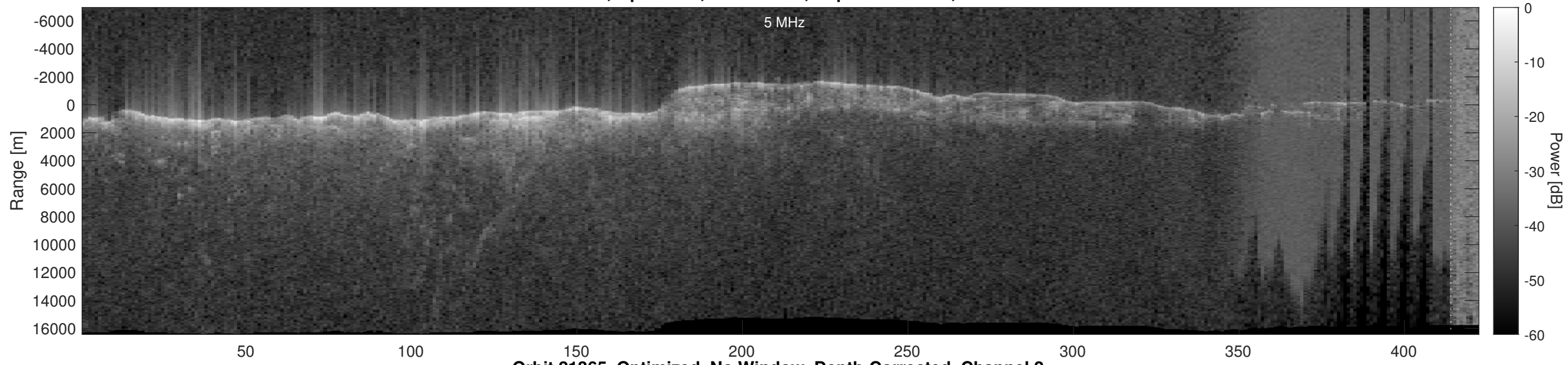
Orbit 21365, Optimized, No Window, Depth-Corrected, Channel 2
