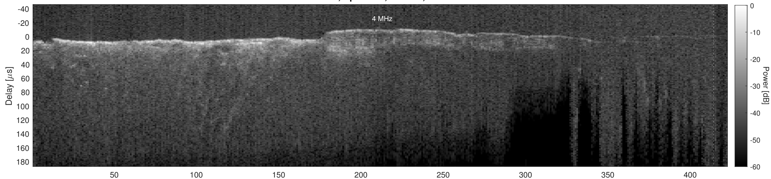
Orbit 21365, Cluttergram
