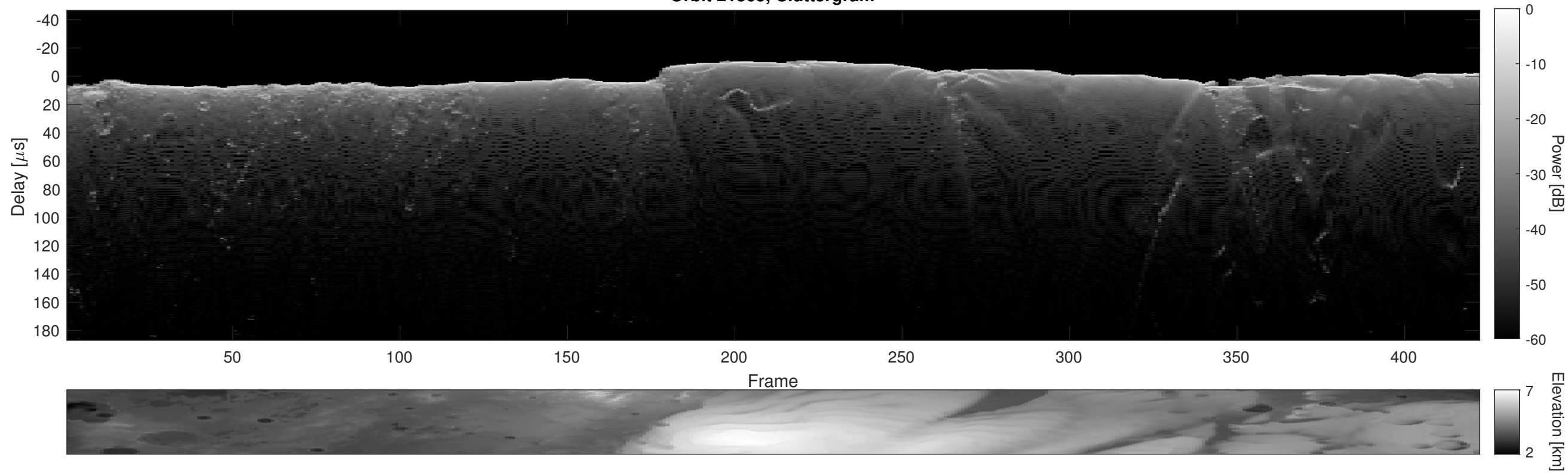
Orbit 21365, Cluttergram
