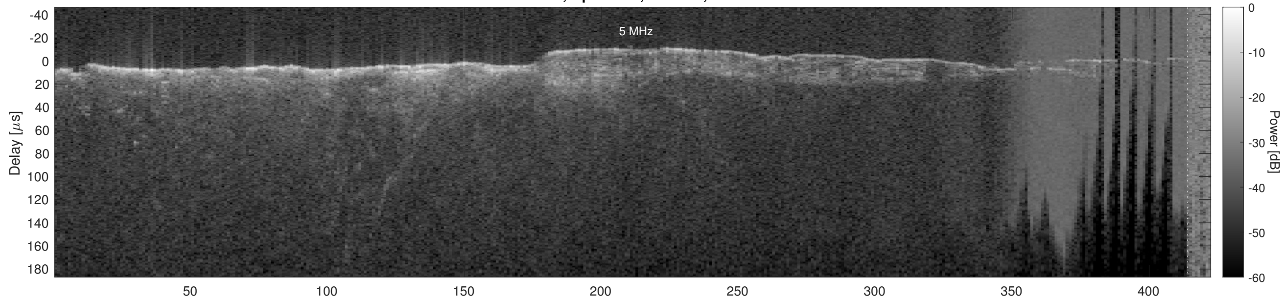
Orbit 21365, Optimized, Window, Channel 2
