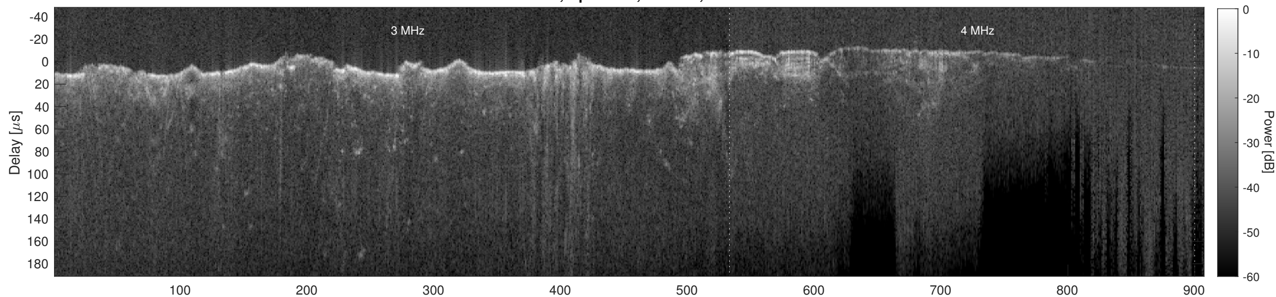
Orbit 21374, Cluttergram
