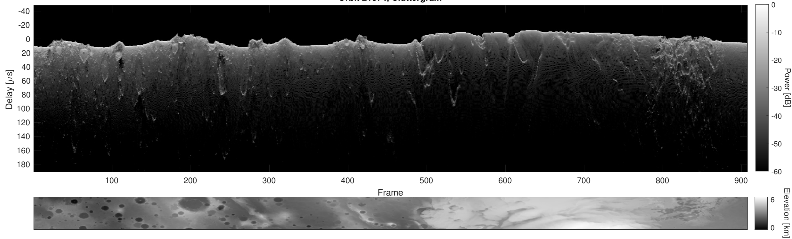
Orbit 21374, Cluttergram
