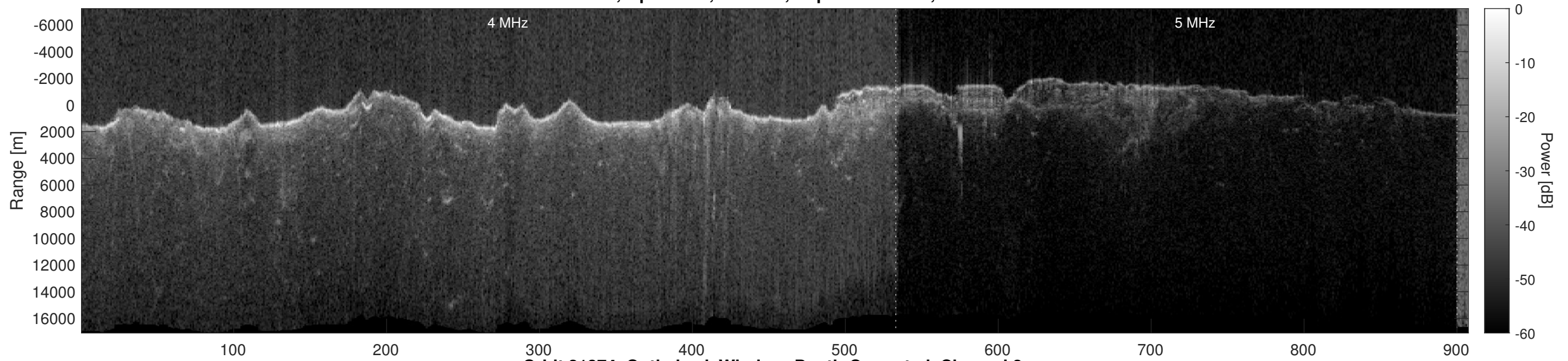
Orbit 21374, Optimized, Window, Depth-Corrected, Channel 2
