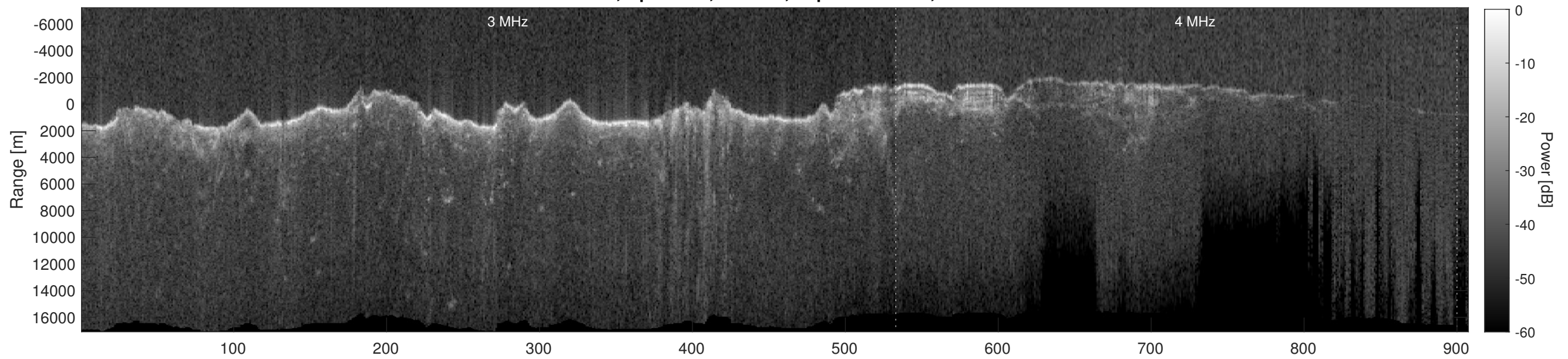
Orbit 21374, Depth-Corrected Cluttergram
